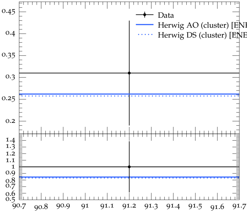
Mean f_2(1270) multiplicity
