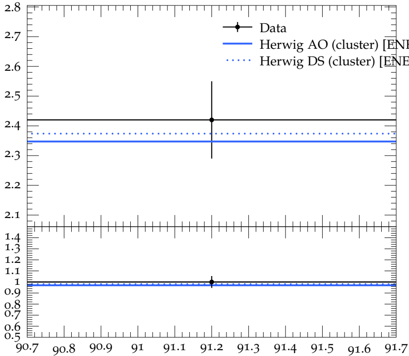
Mean K^+ / K^- multiplicity
