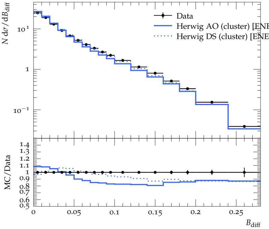
Difference in hemisphere broadening, B_{\text{diff}}
