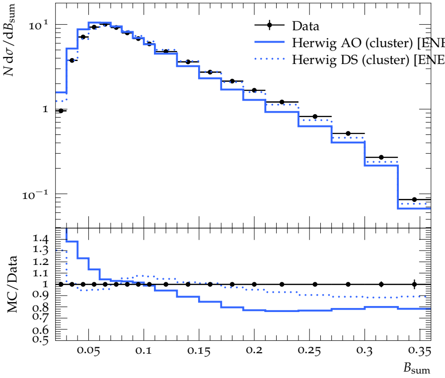
Total hemisphere broadening, B_{\text{sum}}
