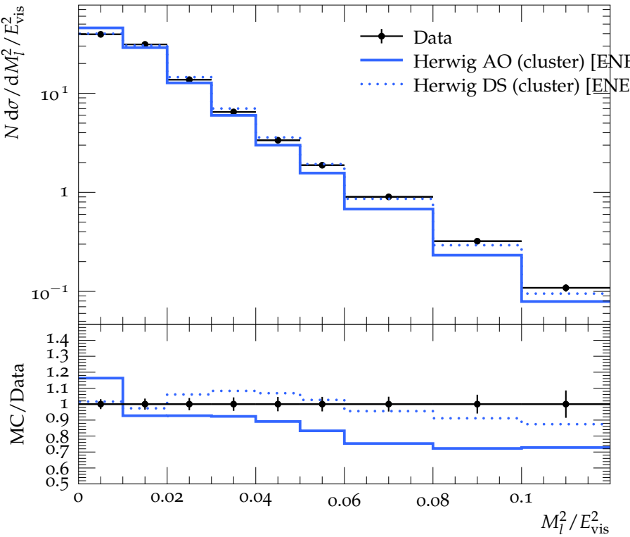
Light hemisphere masses, M_l^2/E_{\text{vis}}^2
