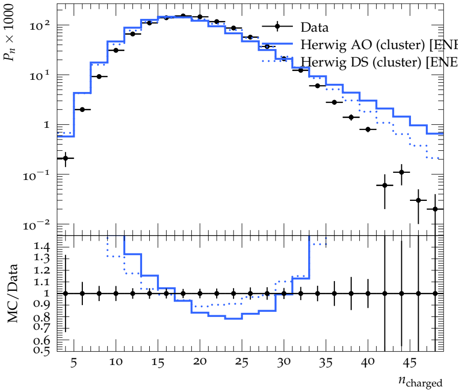
Charged particle multiplicity, 2-jets, y_{\text{cut}} = 0.04
