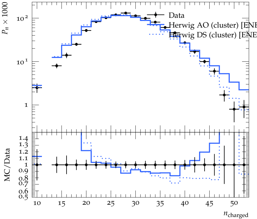
Charged particle multiplicity, 4-jets, y_{\text{cut}} = 0.02
