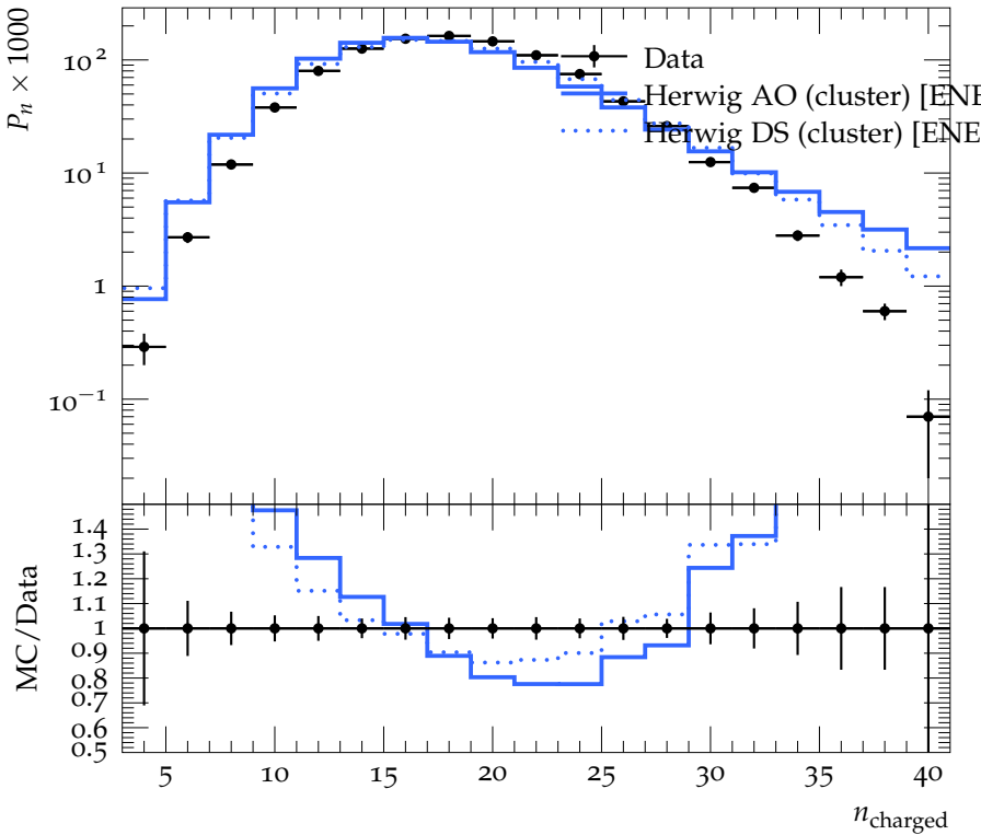
Charged particle multiplicity, 2-jets, y_{\text{cut}} = 0.02
