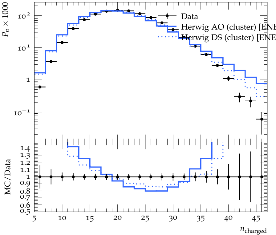
Charged particle multiplicity, 3-jets, y_{\text{cut}} = 0.01
