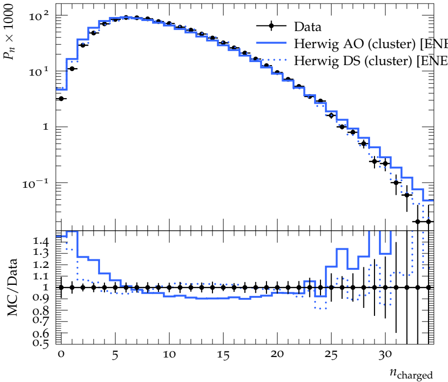
Charged Particle Multiplicity, single hemisphere, |y| < 3.0
