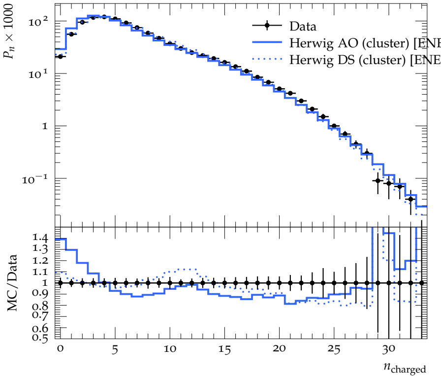
Charged Particle Multiplicity, single hemisphere, |y| < 2.0
