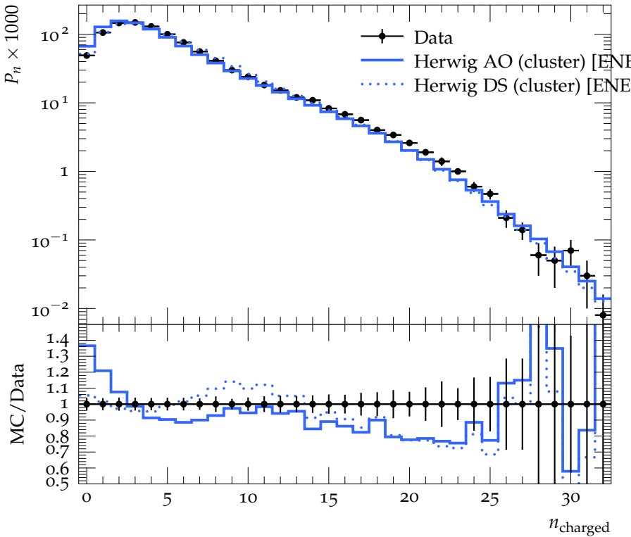
Charged Particle Multiplicity, single hemisphere, |y| < 1.5
