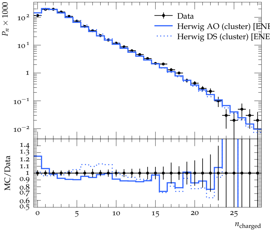
Charged Particle Multiplicity, single hemisphere, |y| < 0.5
