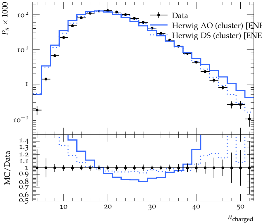
Charged Particle Multiplicity, both hemispheres
