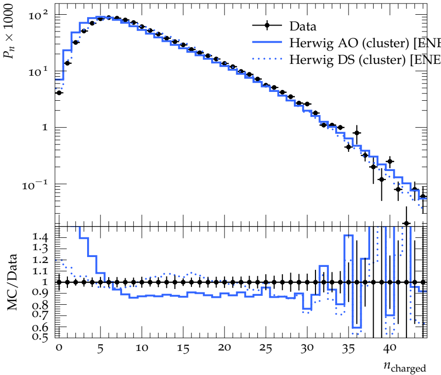
Charged Particle Multiplicity, both hemispheres, |y| < 1.5
