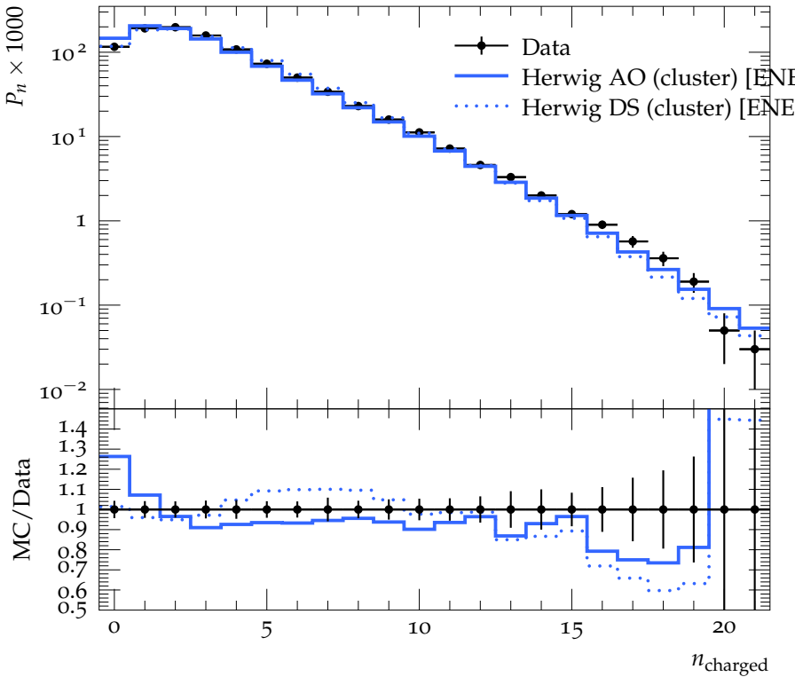
Charged Particle Multiplicity, both hemispheres, |y| < 0.5
