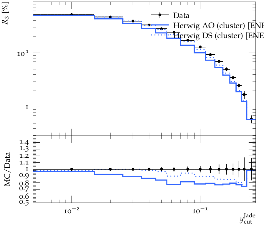
Integrated 3-jet rate with Jade algorithm
