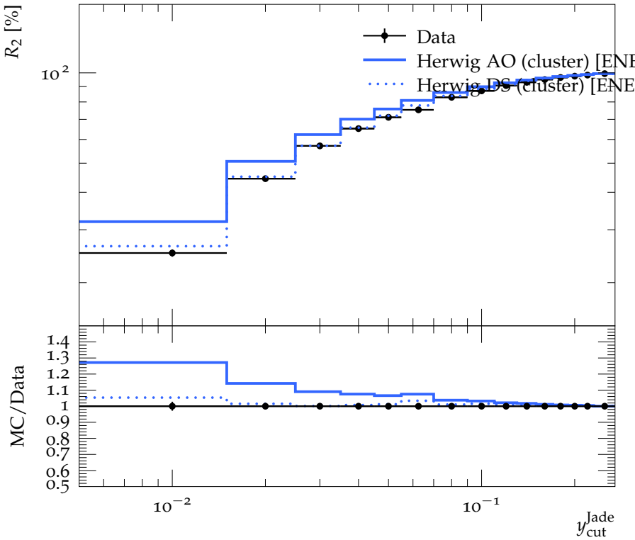
Integrated 2-jet rate with Jade algorithm
