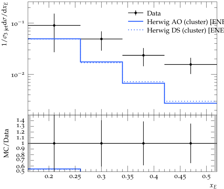
Scaled energy fraction for \eta' in 2nd jet (3-jet events)
