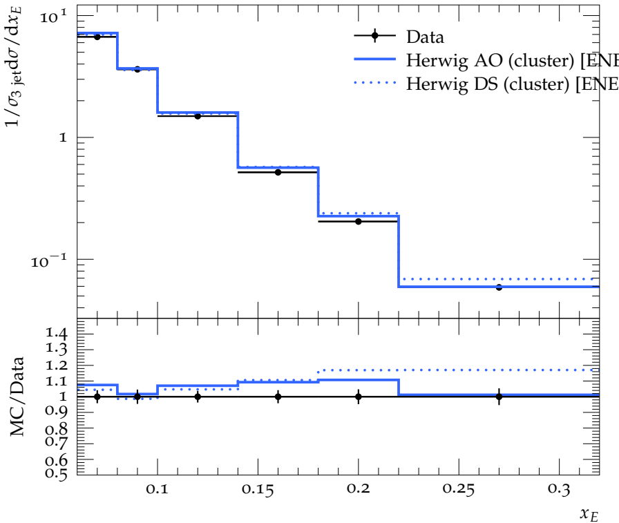
Scaled energy fraction for \pi^0 in 3rd jet (3-jet events)
