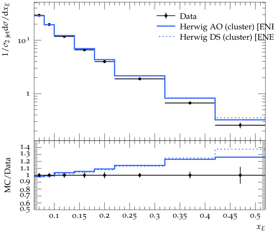
Scaled energy fraction for \pi^0 (2-jet events)
