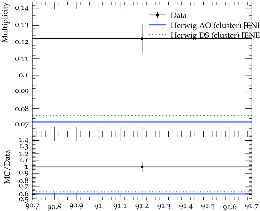
Mean \phi multiplicity
