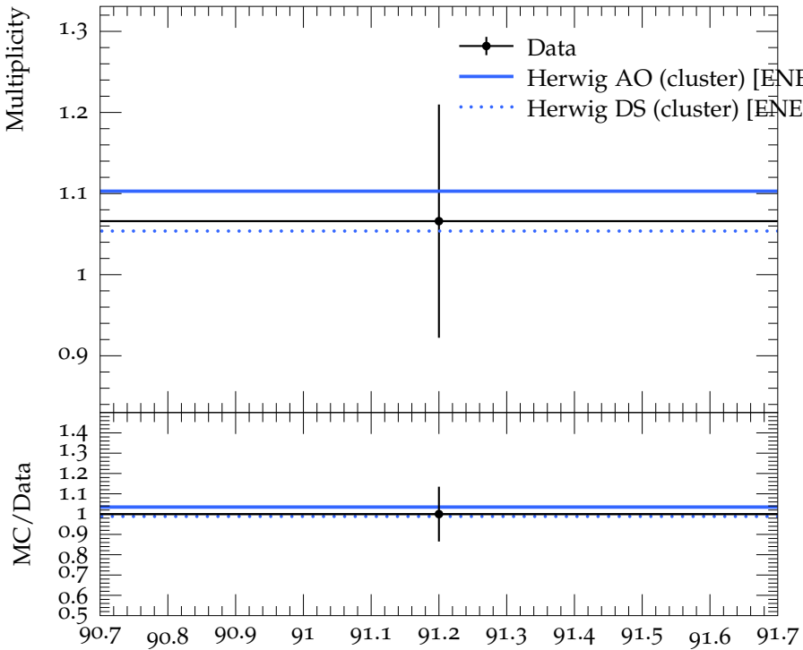
Mean \omega(782) multiplicity
