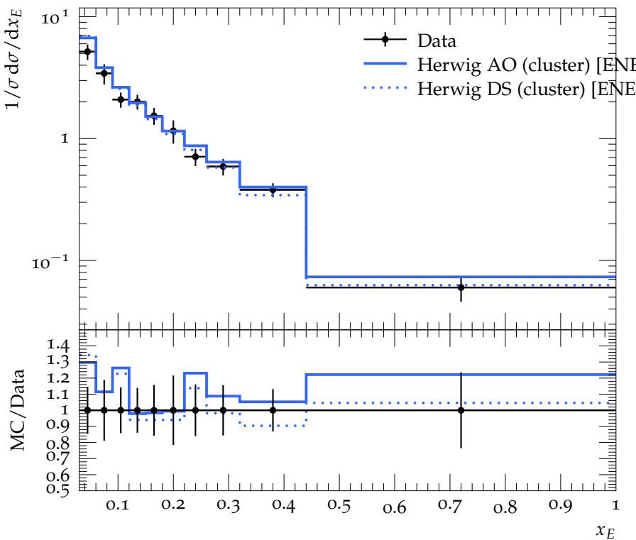
K^{*\pm}(892) spectrum
