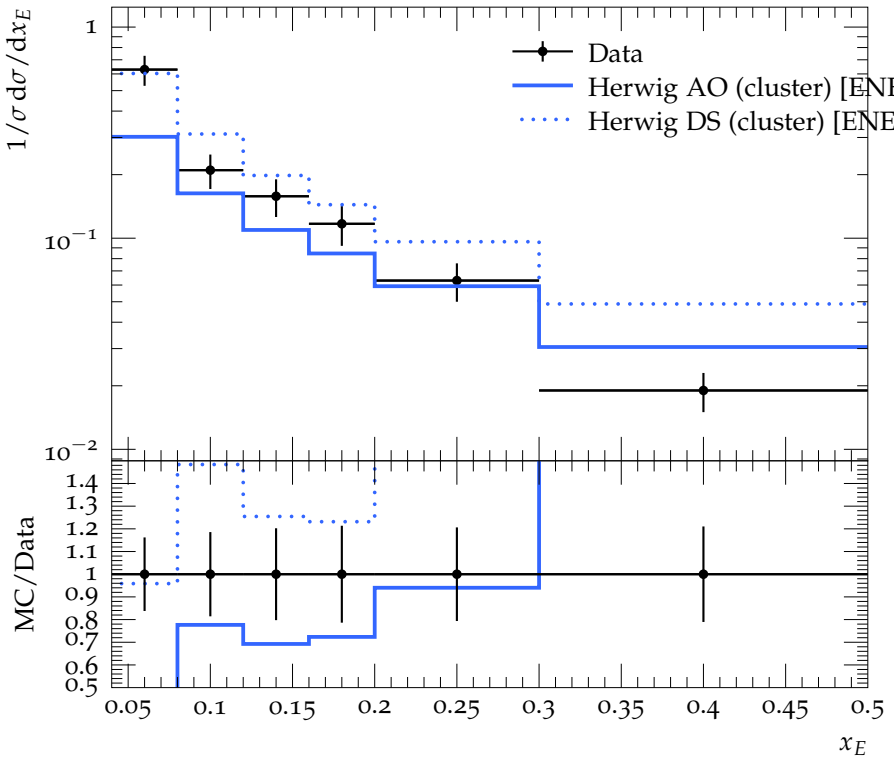
\Sigma^\pm(1385) spectrum
