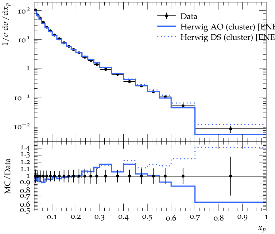
\pi^0 spectrum
