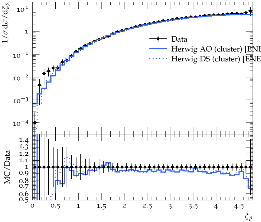
\gamma spectrum
