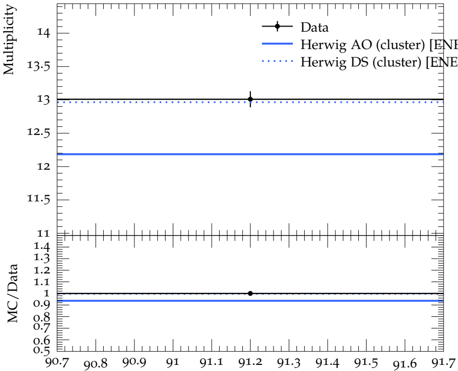
Mean charged multiplicity for rapidity |Y| < 2.0
