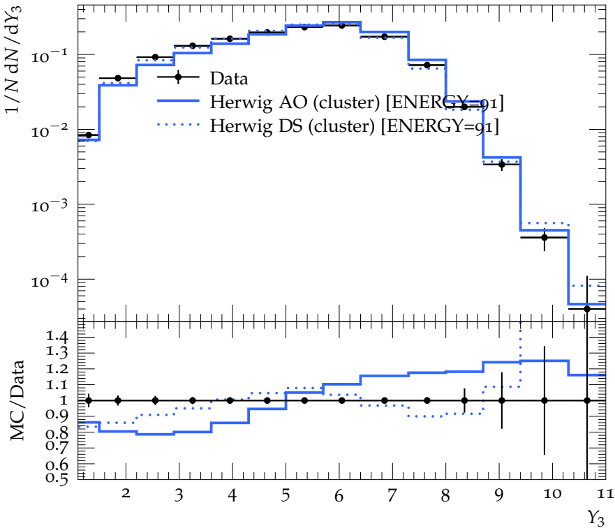
Two-jet resolution variable, Y_3 (charged)
