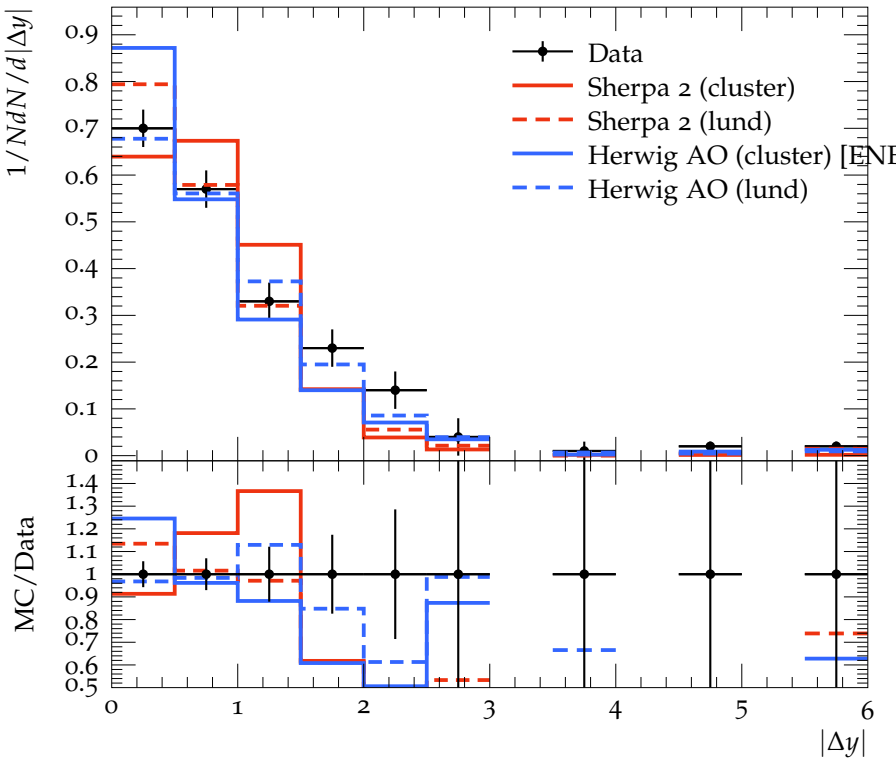
\Lambda\bar{\Lambda} correlation (2 jet events)
