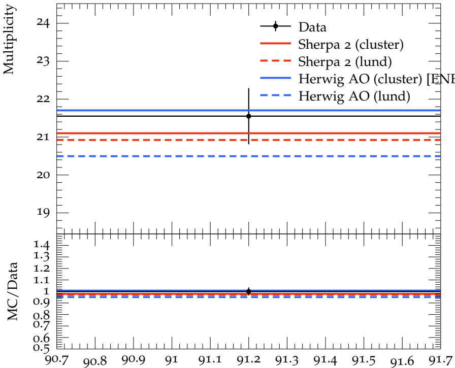
c events mean charged multiplicity
