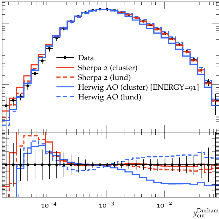
Integrated 4-jet rate with Durham algorithm (91.2 GeV)
