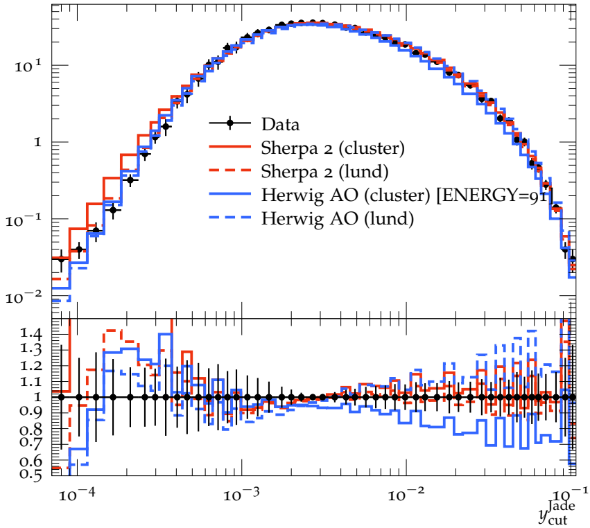
Integrated 4-jet rate with Jade algorithm (91.2 GeV)
