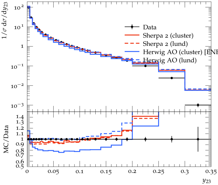
Differential 2-jet rate(Durham)
