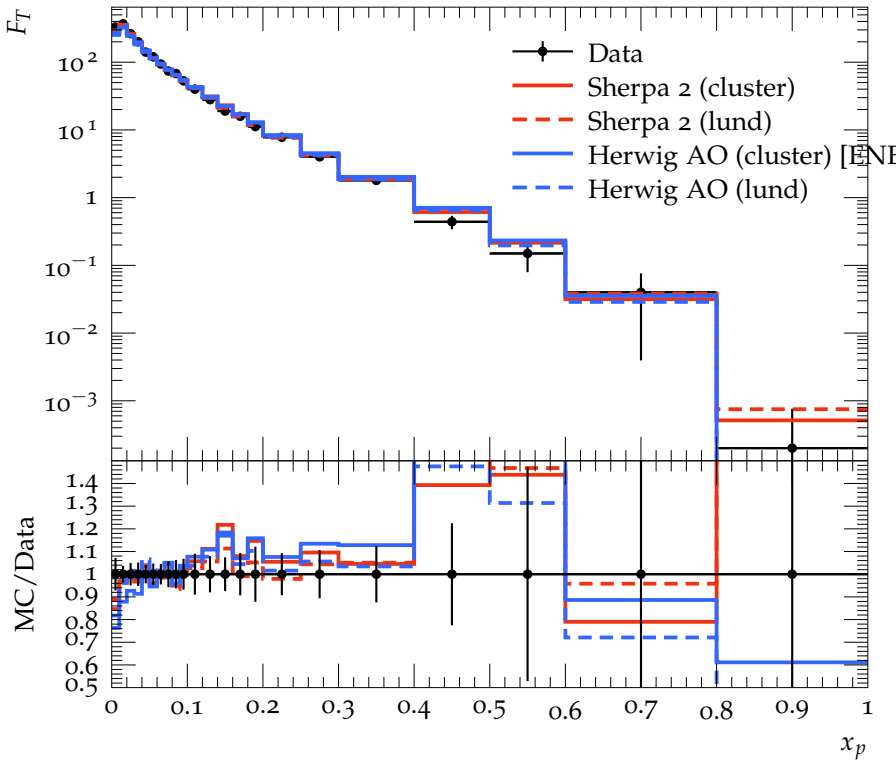
Transverse charged particle fragmentation function (bottom)
