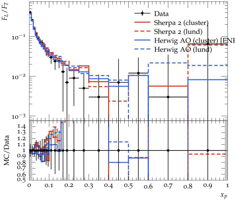
Ratio of Longitudinal and Transverse fragmentation function
