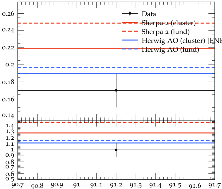
Mean D^*(2010)^+/D^*(2010)^- multiplicity
