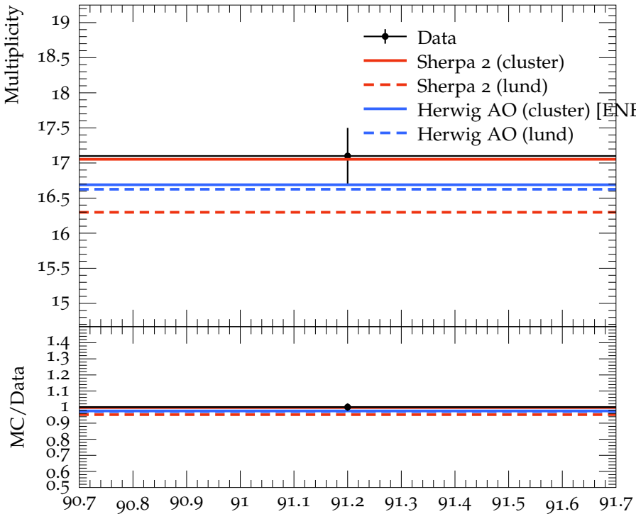
Mean \pi^+/\pi^- multiplicity
