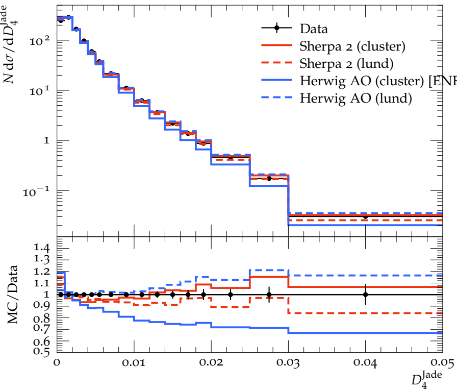
Differential 5-jet rate with Jade algorithm, D_4^{\text{Jade}}
