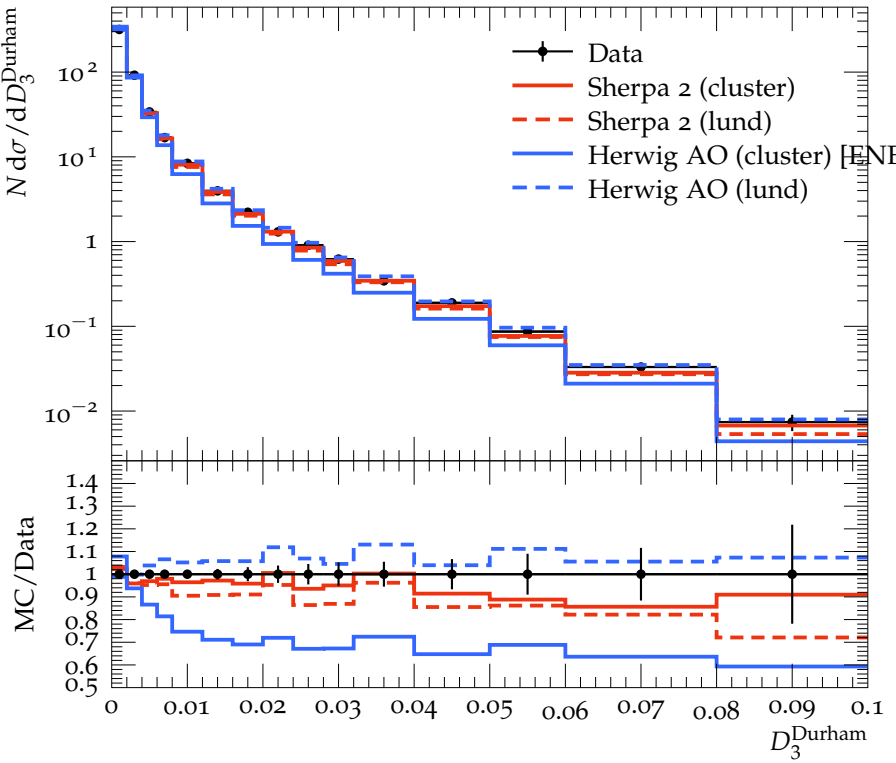
Differential 4-jet rate with Durham algorithm, D_3^{\text{Durham}}
