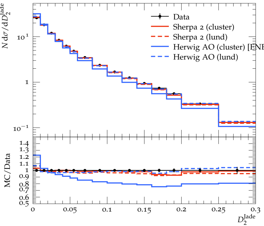
Differential 3-jet rate with Jade algorithm, D_2^{\text{Jade}}
