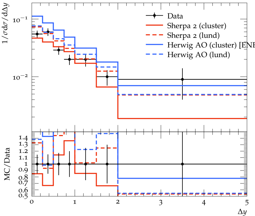
\Lambda^0 and \bar{\Lambda}^0 rapidity difference
