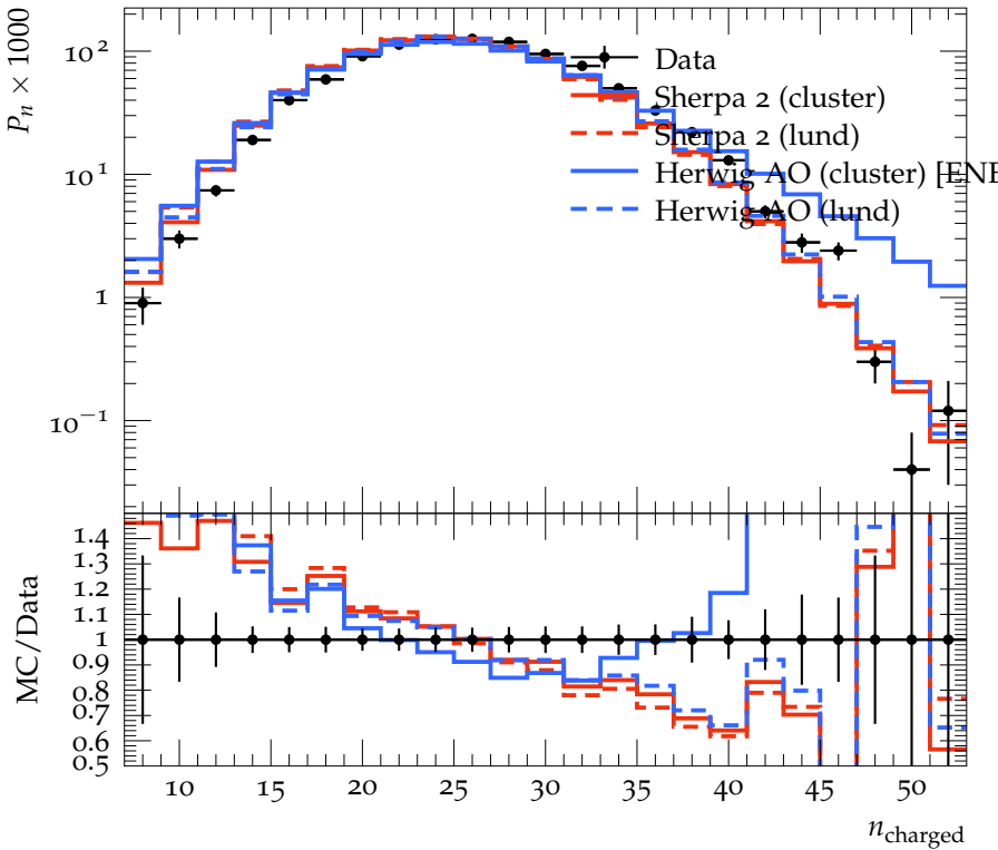
Charged particle multiplicity, 4-jets, y_{\text{cut}} = 0.01
