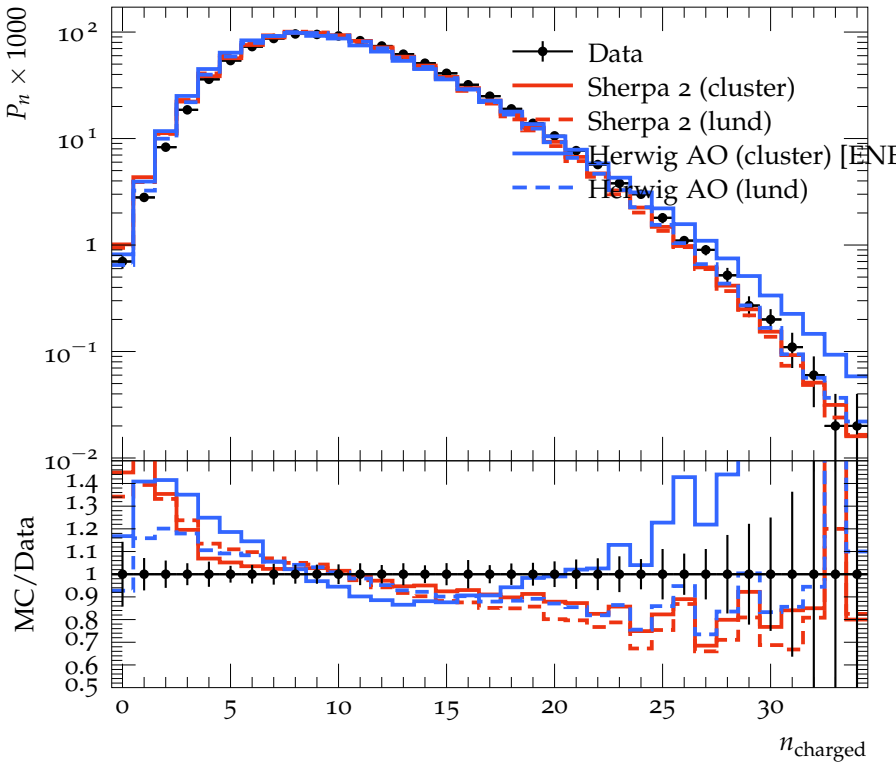
Charged Particle Multiplicity, single hemisphere, |y| < 4.0
