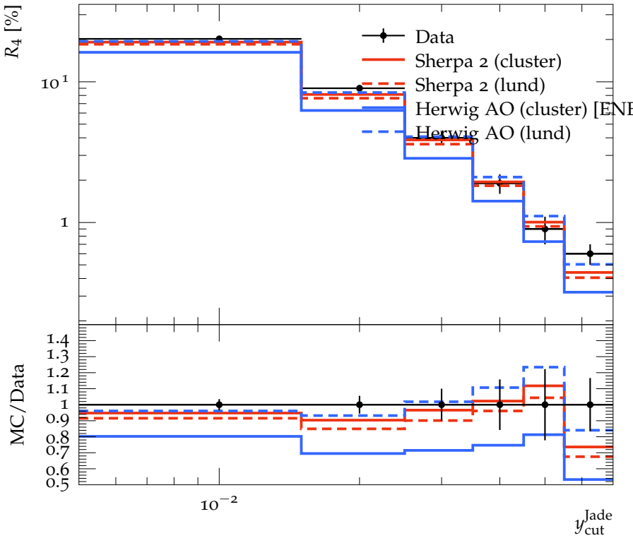
Integrated 4-jet rate with Jade algorithm
