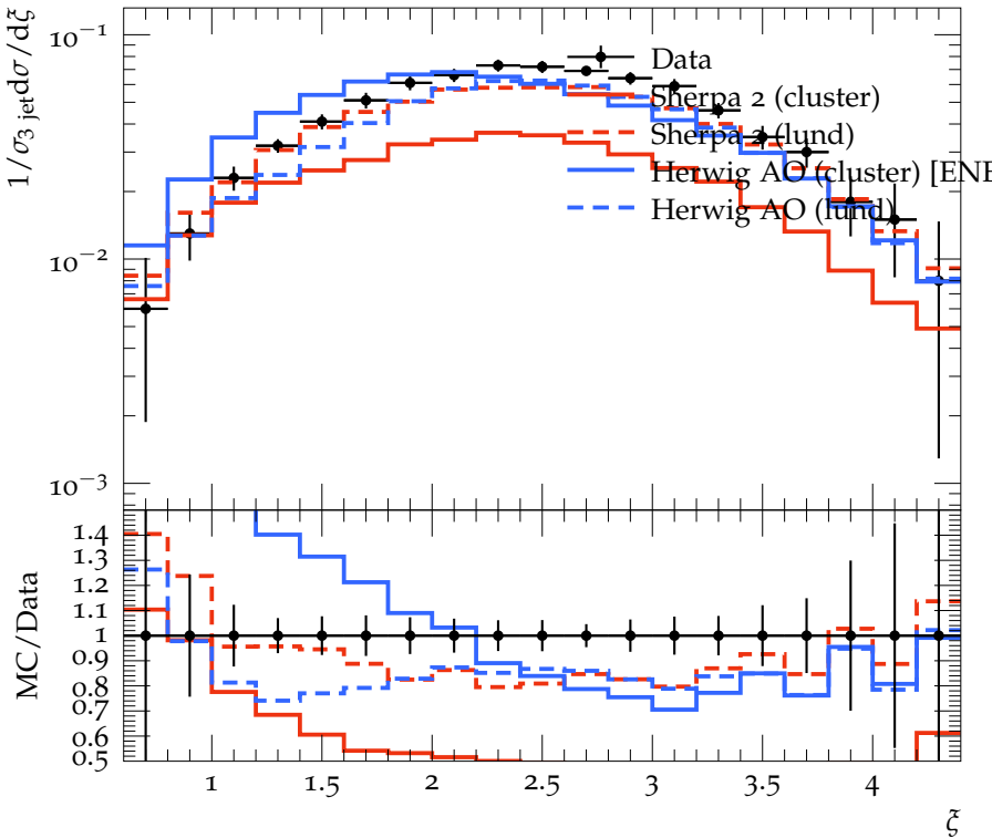
Log Scaled momentum fraction for \Lambda^0 in 2nd jet (3-jet events)
