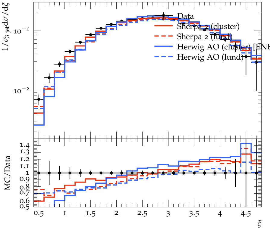
Log Scaled momentum fraction for K_S^0 in 2nd jet (3-jet events)
