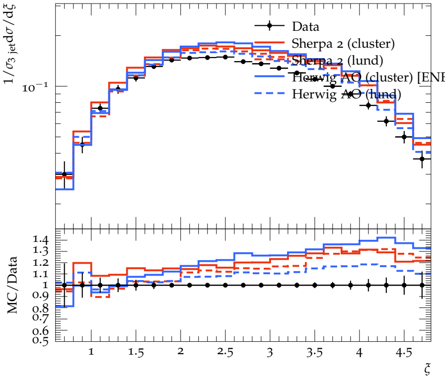
Log Scaled momentum fraction for K_S^0 in 1st jet (3-jet events)
