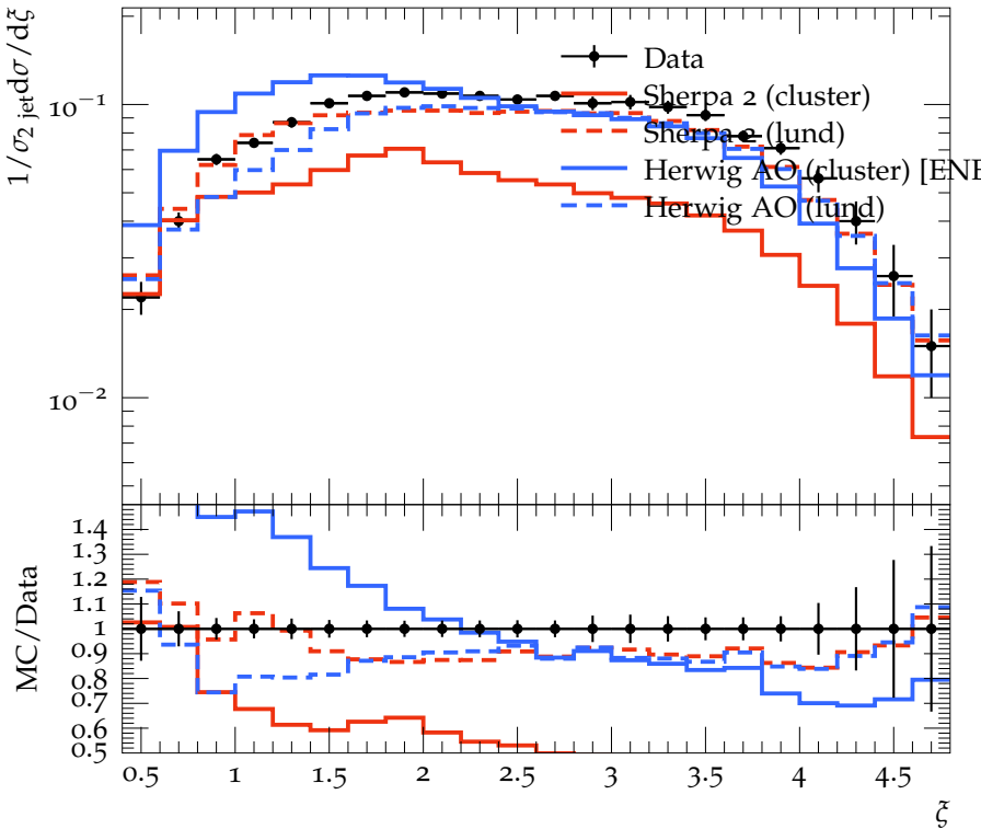
Log Scaled momentum fraction for \Lambda^0 (2-jet events)
