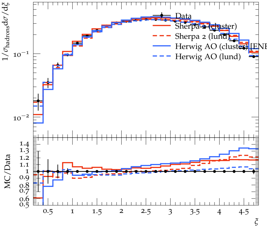
Log Scaled momentum fraction for K_S^0 (all events)
